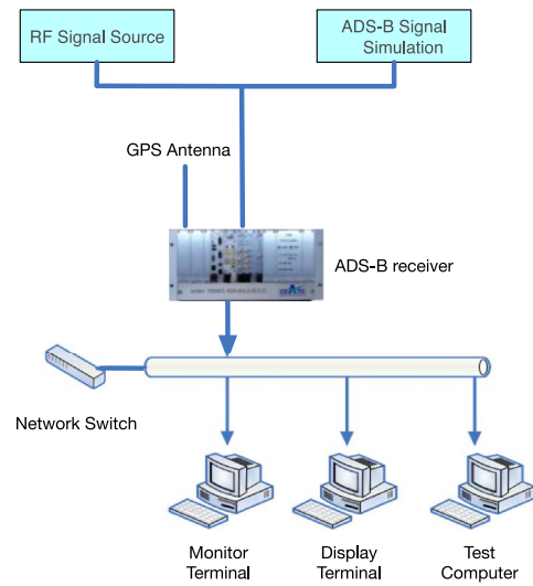
Fig. 11. Test environment.
